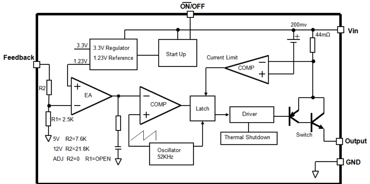
Figure3. Function Block Diagram of HS2576
