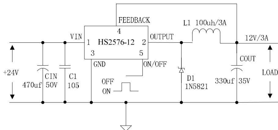
Figure7. HS2576-12 System Parameters Test Circuit
