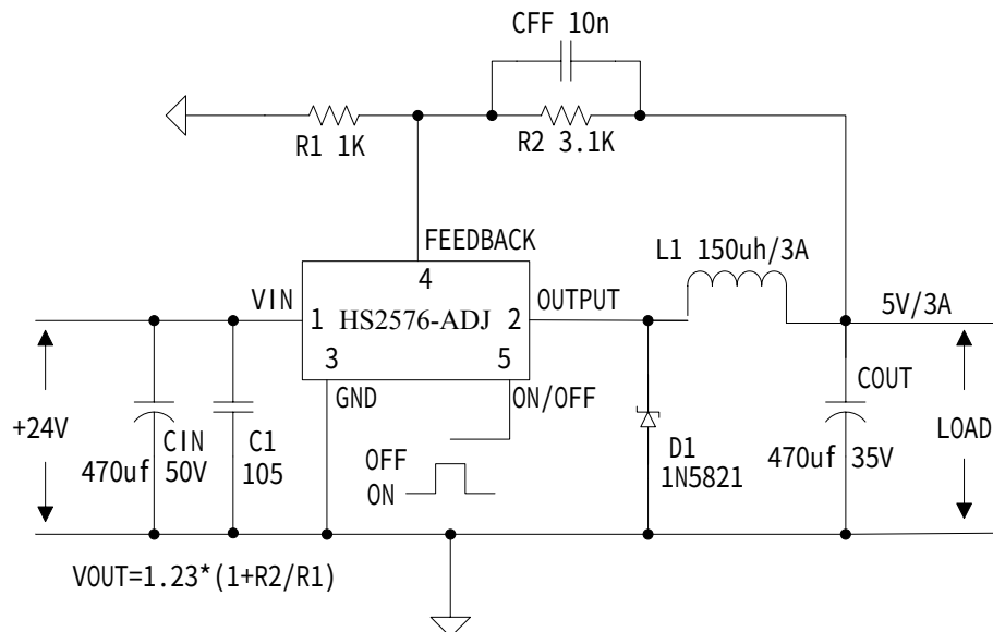
Figure8. HS2576-ADJ System Parameters Test Circuit
