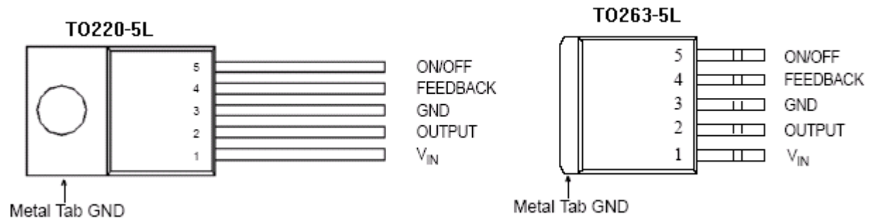
Figure2. Pin Configuration of HS2576 (Top View)
