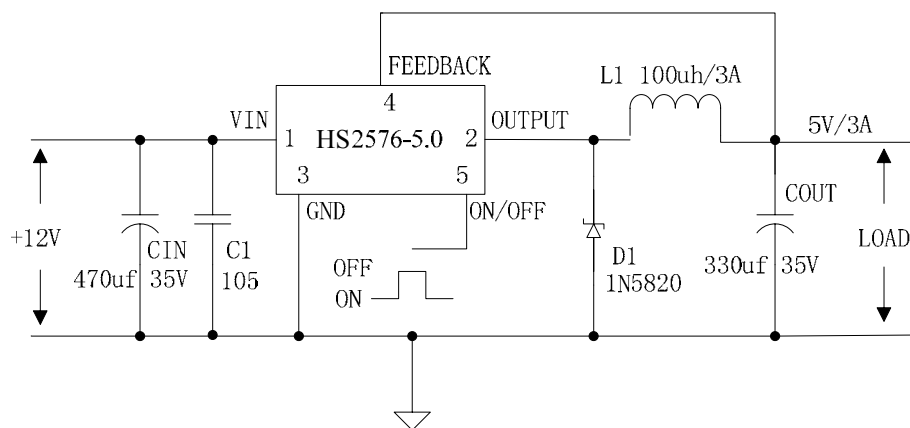
Figure4. HS2576 Typical Application Circuit 12V-5V/3A
