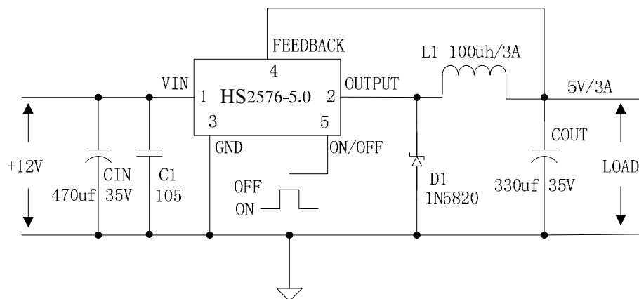
Figure6. HS2576-5.0 System Parameters Test Circuit
